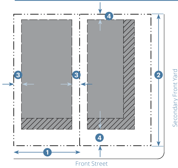
Figure 11.030.5: Determining the Required Amount Subject to the Facade Zone
