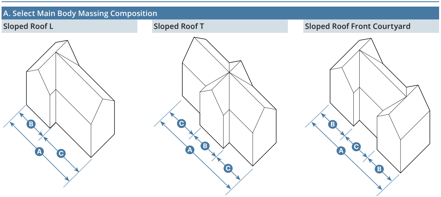
Figure 11.030.15: Example of Massing Type and Bays
