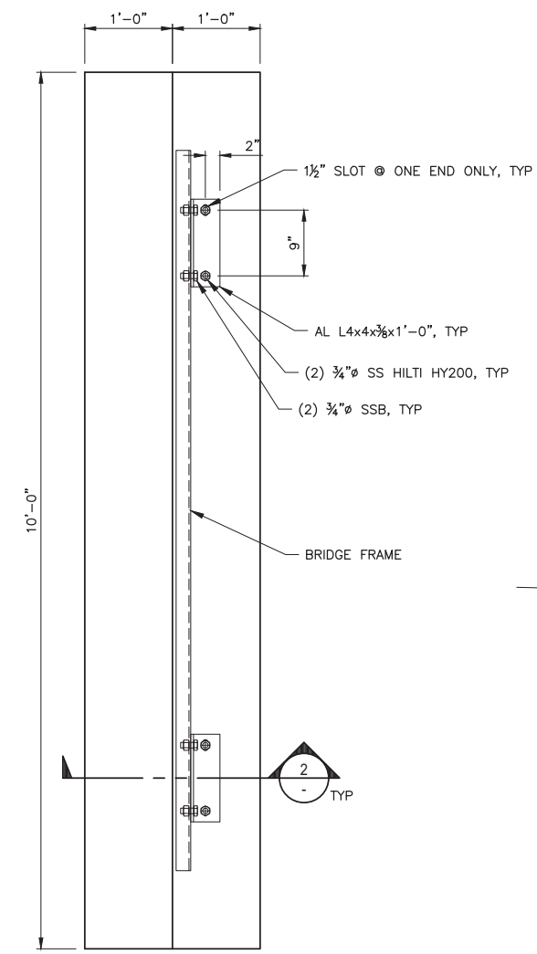
ABUTMENT PLAN SCALE: 1"=1'-0"
